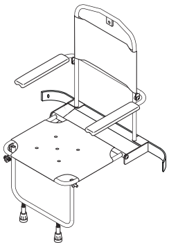
Tip-up PVC shower seat, with folding legs/arms/ fixed backrest
