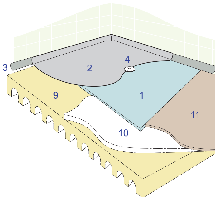
Floating Floor
